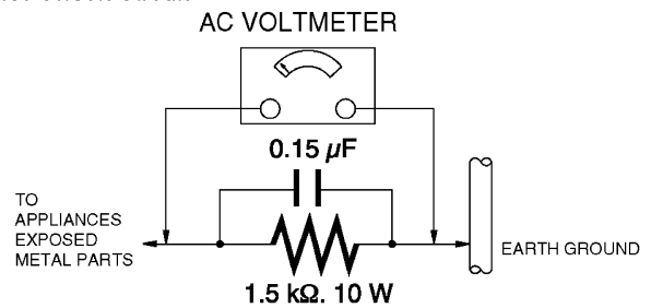
Hot-Check Circuit
